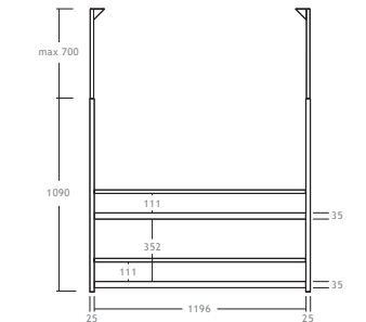
MENSOLA PORTA BOTTIGLIE A SOFFITTO CEILING BOTTLE COMPARTMENT
