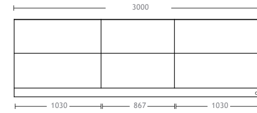
BANCO BAR NEUTRO L3000 H950 P825MM AMBIENT BAR COUNTER W3000 H950 P825MM
