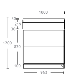
BANCO BAR NEUTRO L1000 H1200 P905MM AMBIENT BAR COUNTER W1000 H1200 P905MM
