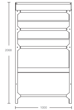
SCAFFALE PANETTERIA A TERRA 1000 P 383 HIGH BAKERY SHELF UNIT 1000 D 383
