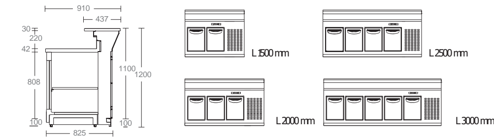
BANCO BAR CON CELLE REFRIGERATE STATICHE E MOTORE INCORPORATO H1200 P825 MM BAR COUNTER WITH STATIC REFRIGERATED ROOMS & HERMETIC UNIT H1200 D825 MM
