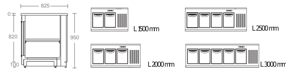
BANCO CON CELLE REFRIGERATE STATICHE E MOTORE INCORPORATO H950 P825 MM COUNTER WITH STATIC REFRIGERATED ROOMS & HERMETIC UNIT H950 D825 MM
