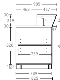
BANCO BAR NEUTRO H1200 P905MM AMBIENT BAR COUNTER H1200 P905MM
