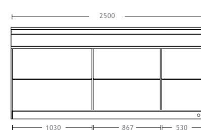
BANCO BAR NEUTRO L2500 H1200 P905MM AMBIENT BAR COUNTER W2500 H1200 P905MM
