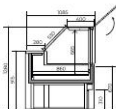
CALDO SECCO _ DRY HEATED Dim: 1000-1500 mm
