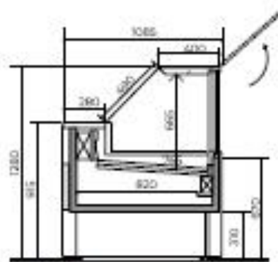
FREDDO STATICO CON CELLA STATIC COLD WITH REFRIGERATED STORAGE Dim: 1600-2000-2500-3000 mm
