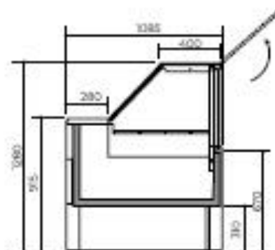
BAGNOMARIA _ BAIN MARIE Dim: 1500 mm
