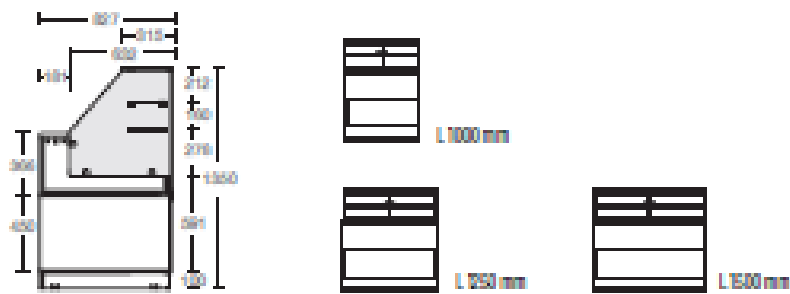
VETRINA PANETTERIA NEUTRO H1350 P1825 MM BAKERY AMBIENT DISPLAY CASE H1350 D827 MM
